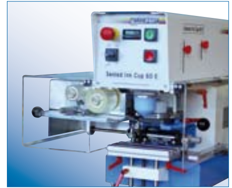
Figure: With integrated ink residue pick-up system
