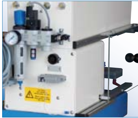
Figure: Rear side with interface SUB-D 37-poles
