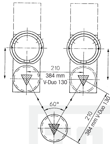
V-60/90 DUO Standard tampon printing machine
